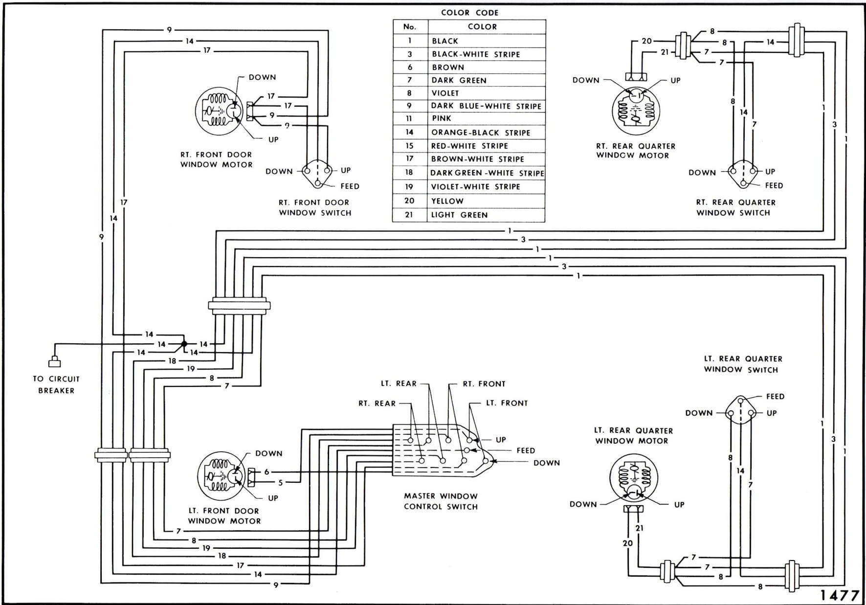
Fig. 2L6—Power Window Circuit Diagram
