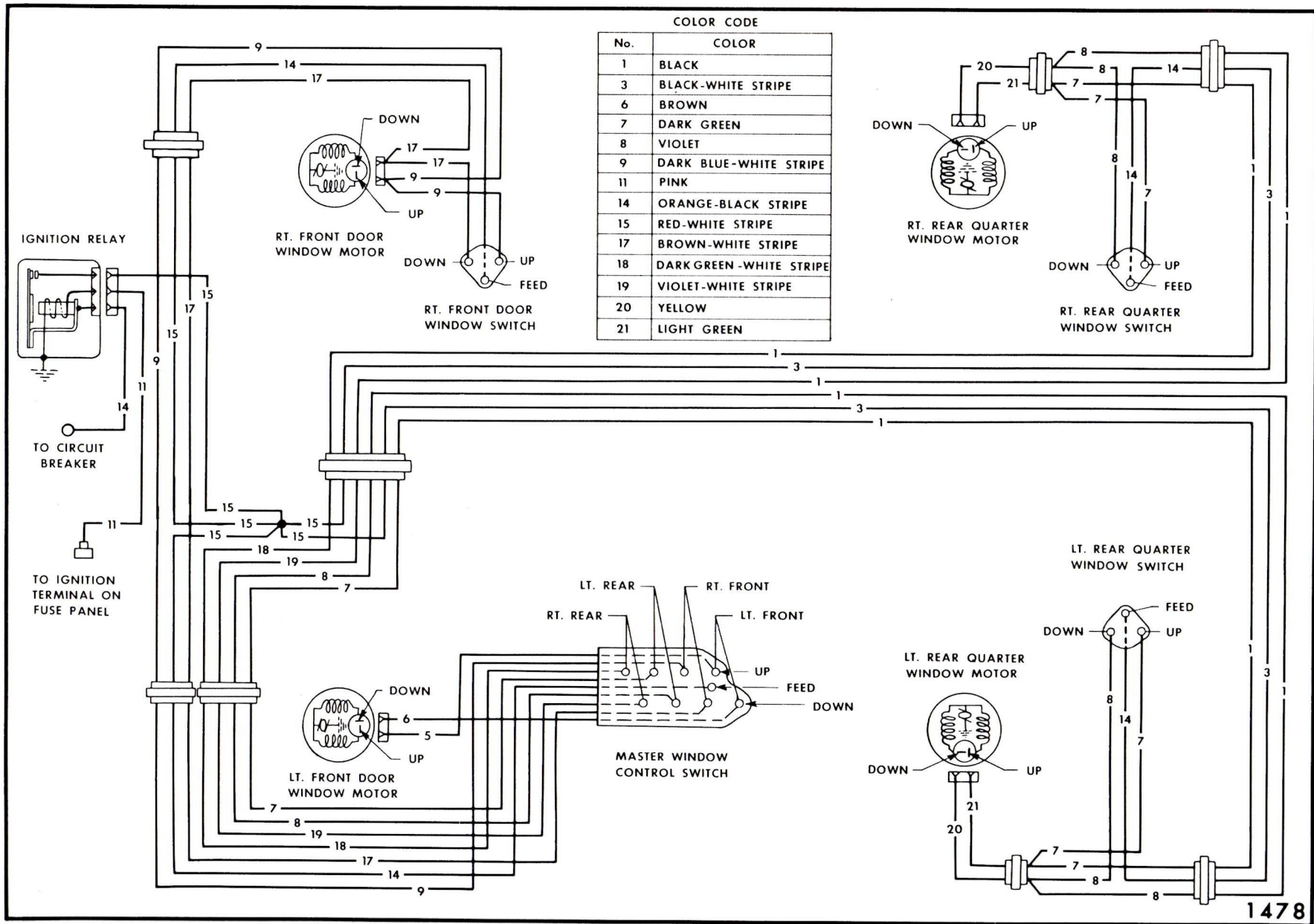
Fig. 217—Power Window Circuit Diagram - 33000 Series
